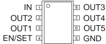
AAT4290A SC70JW-8 (Top View)
