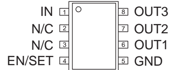
AAT4291A SC70JW-8 (Top View)
